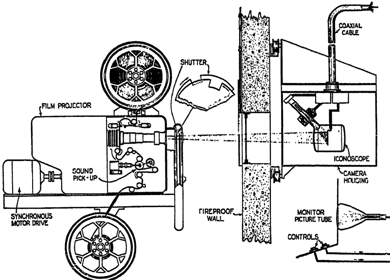
Motion-picture pickup, consisting of a film projector directed into a television camera.
